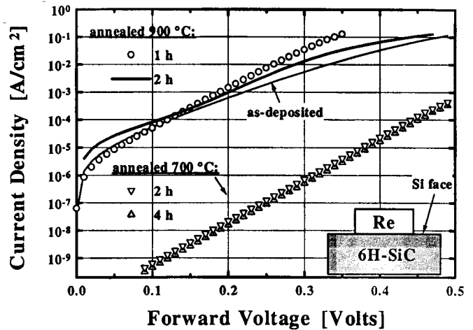
Fig. 2. A semilogarithmic I - V plot of a circular Re contact on the Si face of a 6H-SiC substrate before and after annealing in vacuum for 2 and 4 h at 700\text{ }^\circ\text{C} and for 1 and 2 h at 900\text{ }^\circ\text{C} .
