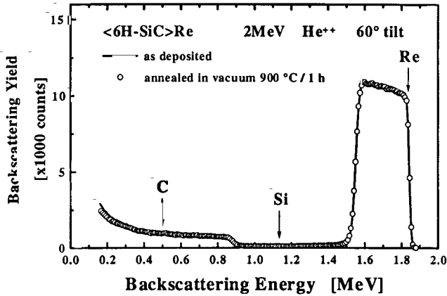
Fig. 1. MeV 4\text{He}^{++} backscattering spectra of a 100-nm thick Re film on 6H-SiC substrate before (solid curve) and after (open circles) annealing in vacuum at 900\text{ }^\circ\text{C} for 1 h. The arrows mark the surface energy of the involved elements. (The angle of the incident beam against the sample normal is 60\text{ }^\circ ; the scattering angle of the detected particles is 165\text{ }^\circ ).
